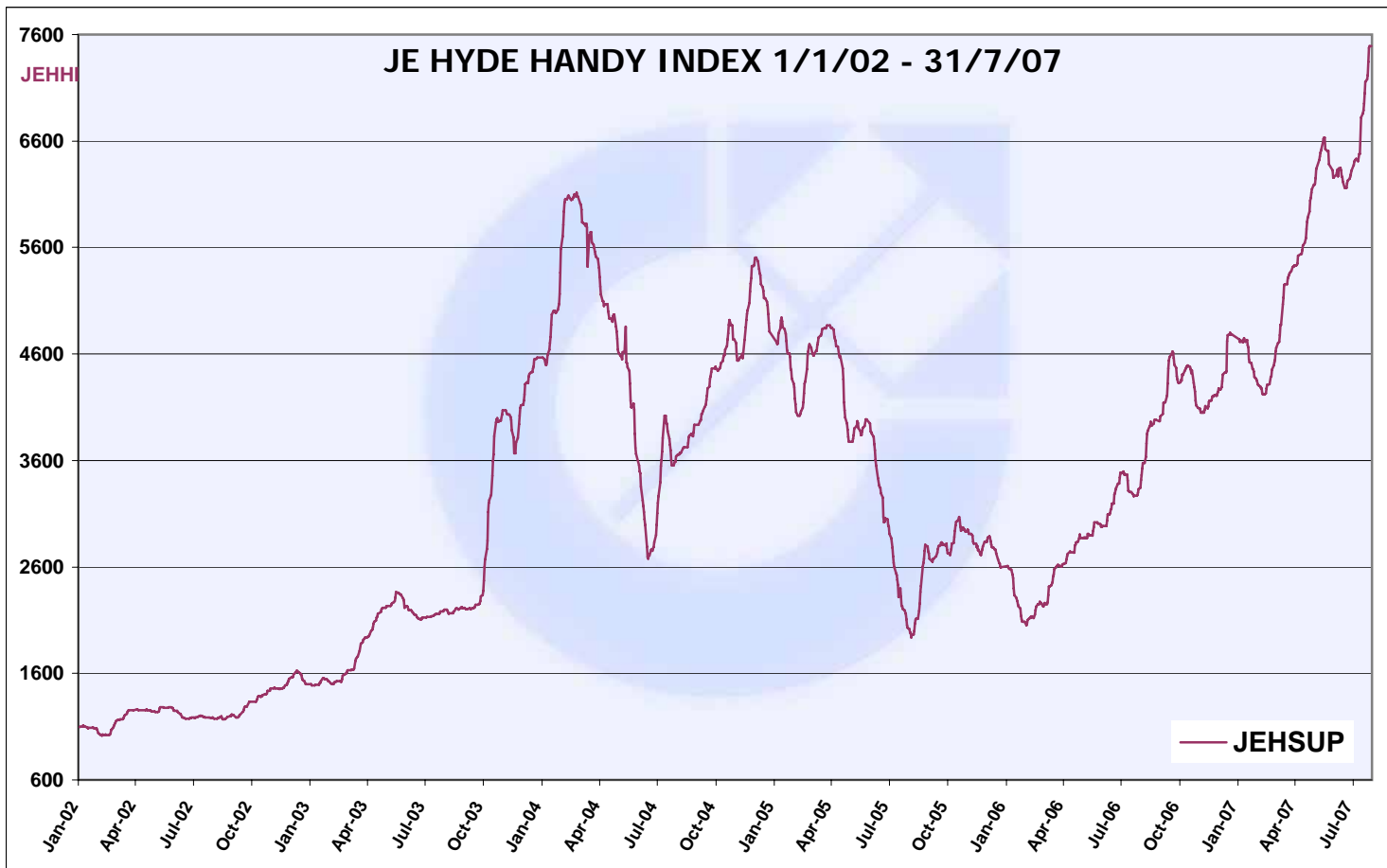
JE HYDE HANDY INDEX 1/1/02 - 31/07/2007 (5 YEARS)
