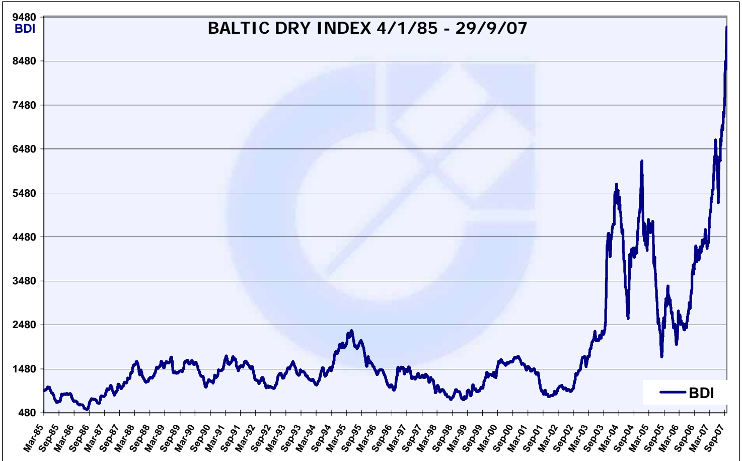
BALTIC DRY INDEX 4/1/85 - 29/09/2007 (22 YEARS)
